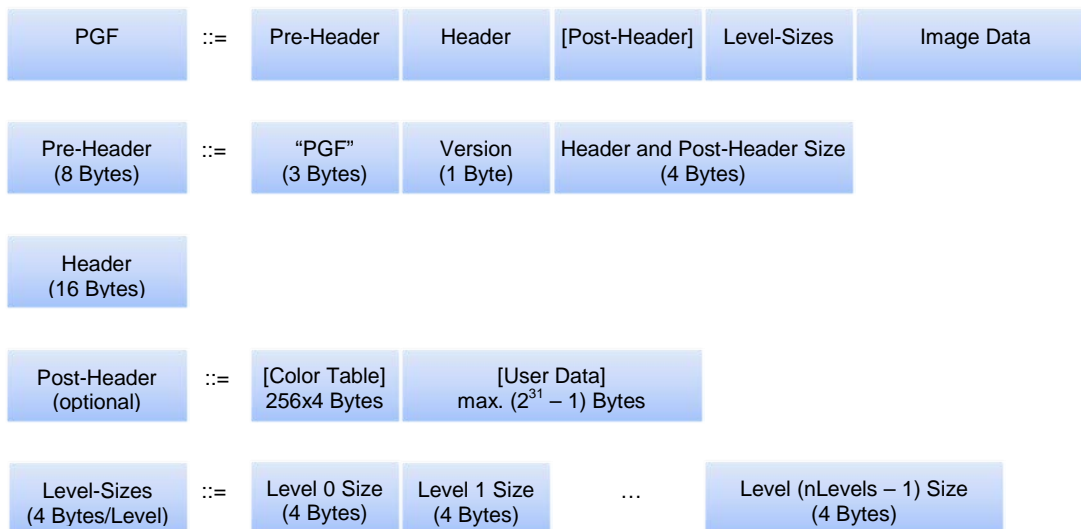
Figure 1: PGF header structure
