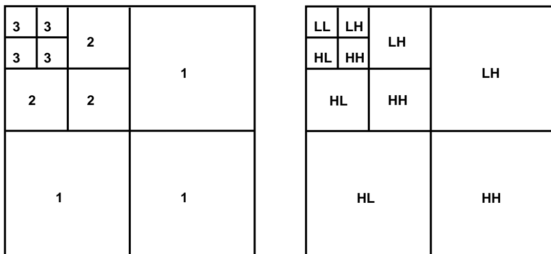
Figure 2: Resolution levels (0 - 3) and DWT pyramid (L: low pass filter, H: high pass filter)
